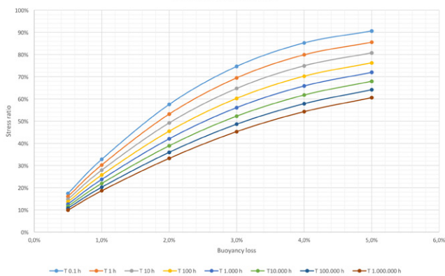
Isocronical stress-strain curves from Hydrostatic compressive creep test (Data > 1000 h are extrapolated)
