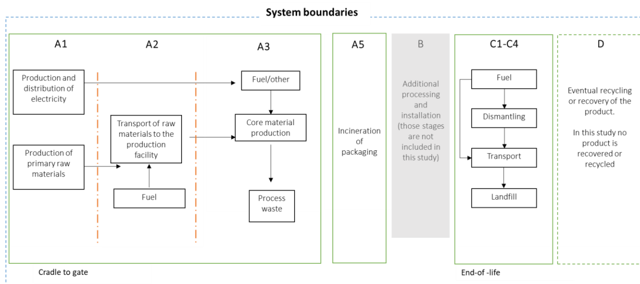
Figure 1. System boundaries of the assessment. The grey box indicates the modules that are excluded from the study.
